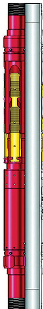
A spacer ring in the IntegraLine S liner hanger prevents rotation after setting.
