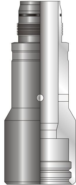
Pickup Sub with Profile for SWP/DWP Wiper Plug
