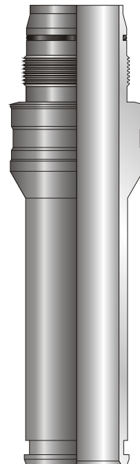
Pickup Sub with Profile for LWP Wiper Plug
