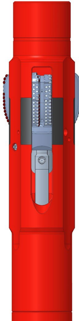
The Weatherford RipTide drilling reamer has retractable and concentric cutter blocks that minimize vibration while drilling and facilitate tool retrieval.
